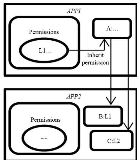
Fig. 1: Access permission architecture (Encket et al. , 2009)
